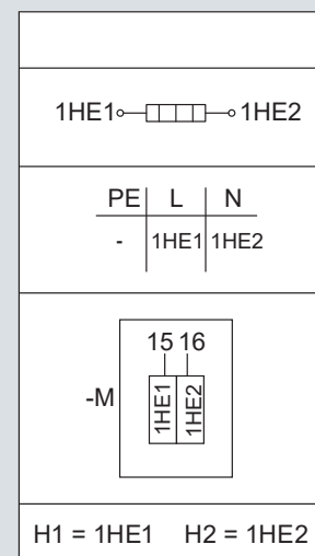
Diagram of connections for anti-condensation heating
