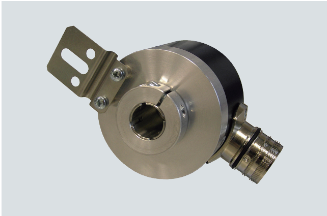
Resolver 1XP8013
