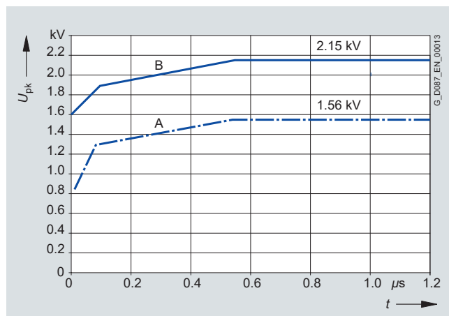
A Standard insulation B Reinforced insulation
